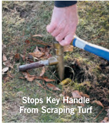
¾" MPT x ½" FPT outlet ¾" FPT inlet Part # QK-075EX
