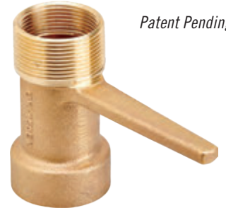
1½" MPT x 1¼" FPT outlet 1½" FPT inlet Part # QK-150EX
